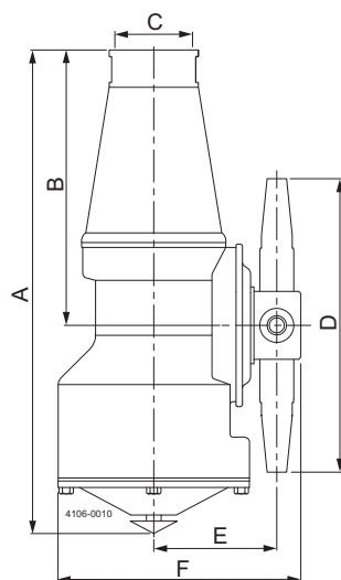
Dimensions (mm)
