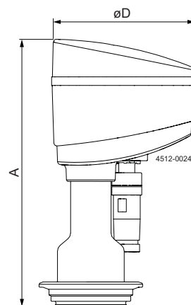
Rotacheck with M12 plug
