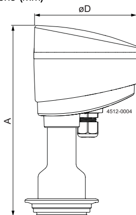
Rotacheck with M16 cable gland
