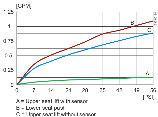
Figure 12. Unique Mixproof Process 3"
