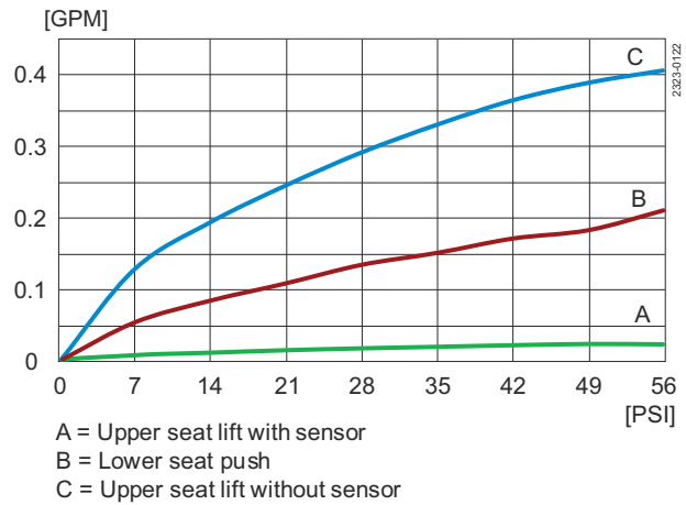
Figure 8. Unique Mixproof Process 2"
