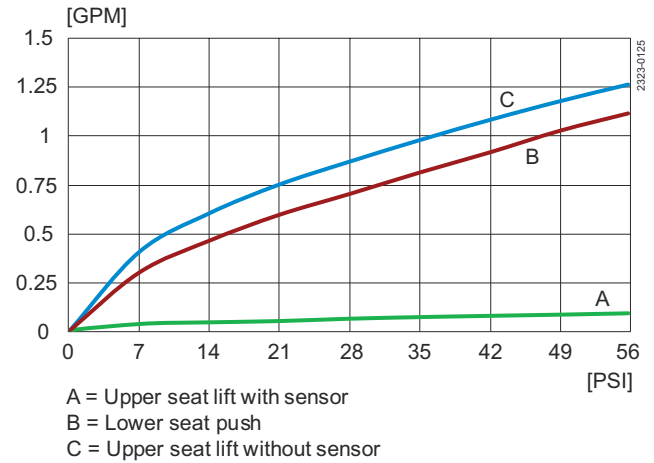
Figure 14. Unique Mixproof Process 4"
