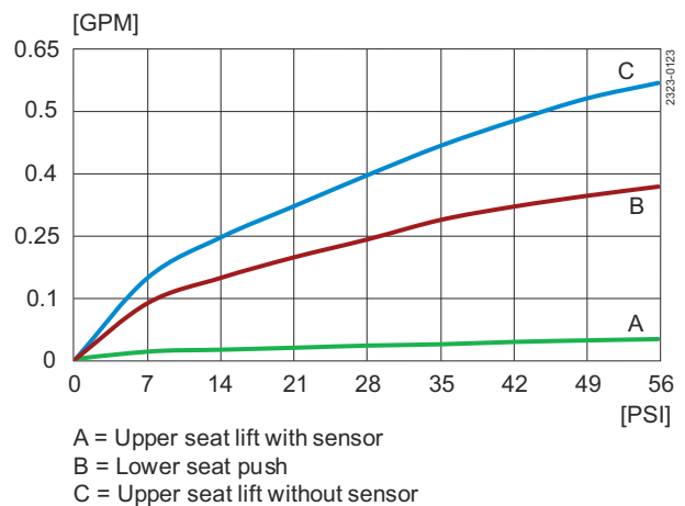
Figure 10. Unique Mixproof Process 2.5"
